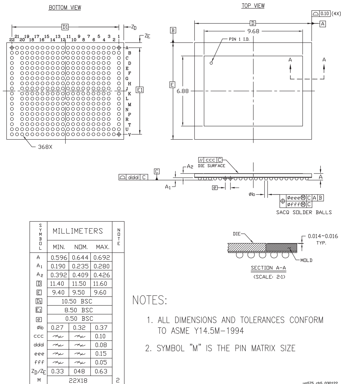
Figure 4-1: Package Dimensions for UBVA368 (XCAU10P and XCAU15P)
